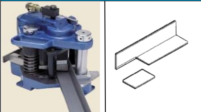
90° 切角 corner cutting
