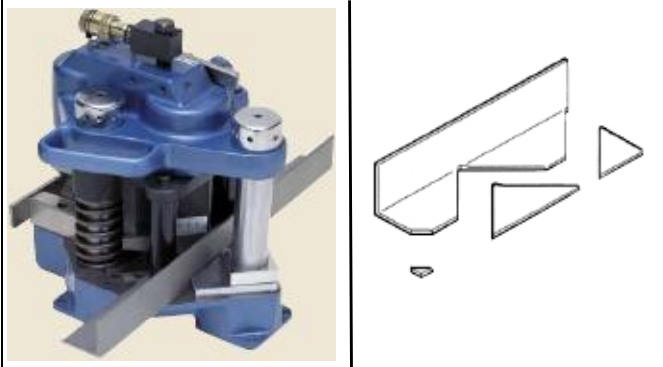
90° V开槽/45° 切角 90° V notching/45° corner cutting
